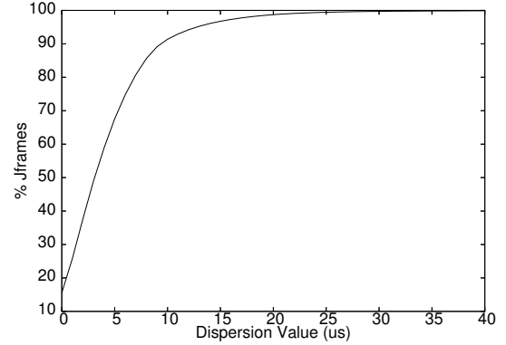
Figure 4: CDF of group dispersion across all frames.
